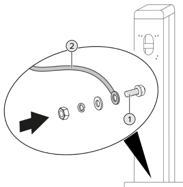
Afb. 3: Product aarden
