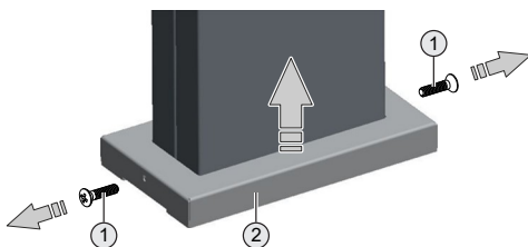
Afb. 4: Afdekking losmaken
