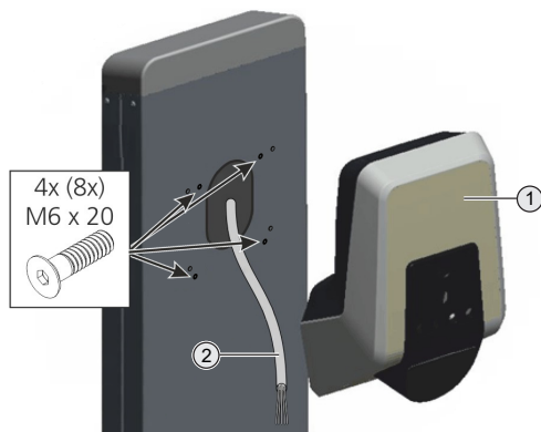
Afb. 6: AMTRON® monteren
