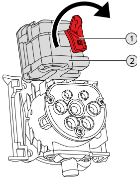
Fig. 24: Unlock the charging plug manually
