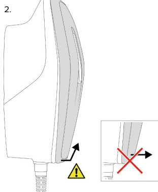
Abb. 5: Front Cover lösen - 2
