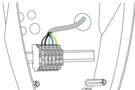
Fig. 10: Power supply connection
