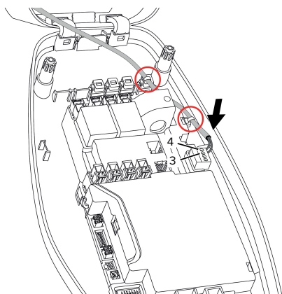
Fig. 14: Tilkobling Downgrade-inngang
