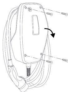
Afb. 6: Product openen
