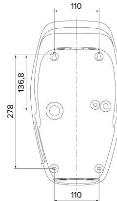
Abb. 8: Bohrmaße [mm]
