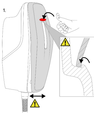
Abb. 20: Front Cover anbringen - 1
