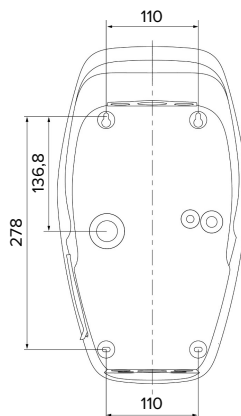
Fig. 8: Drilling dimensions [mm]
