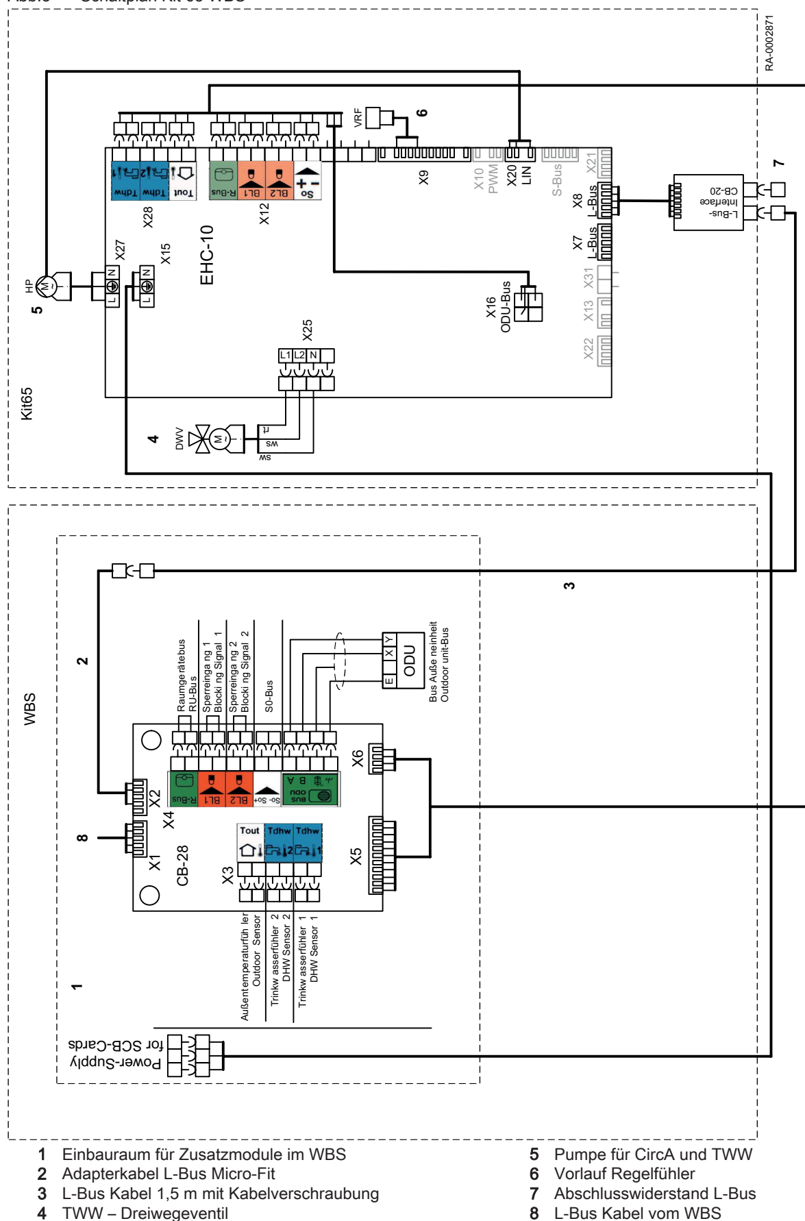
Abb.3 Schaltplan Kit 65 WBS
