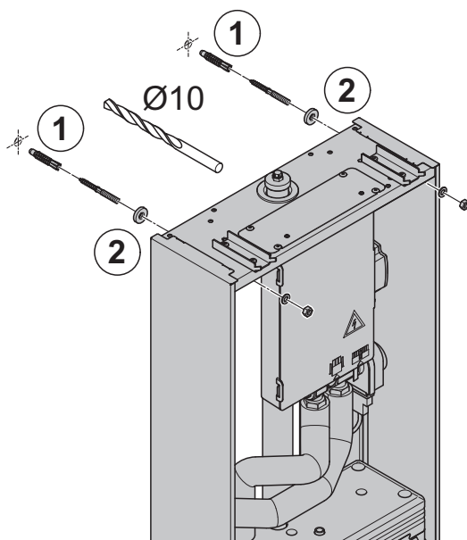
Abb.12 Wandmontage
