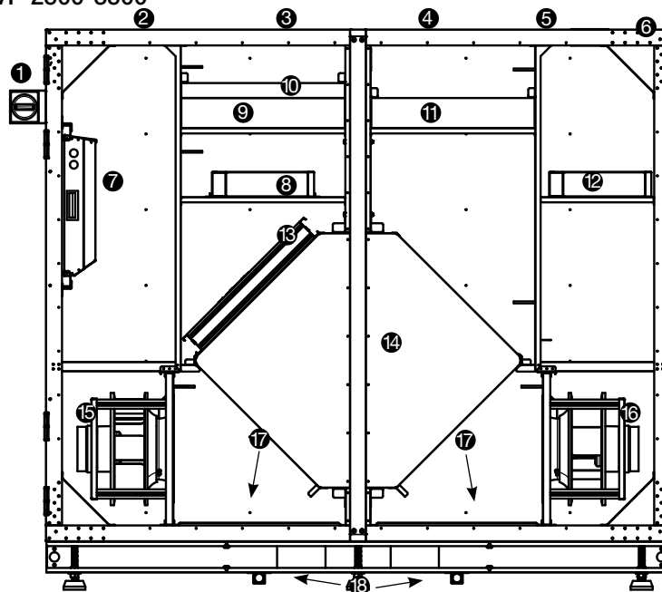
AIR1 XVP 2500-3500
