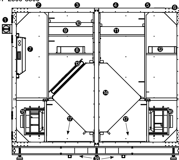
AIR1 XVP 2500-3500
