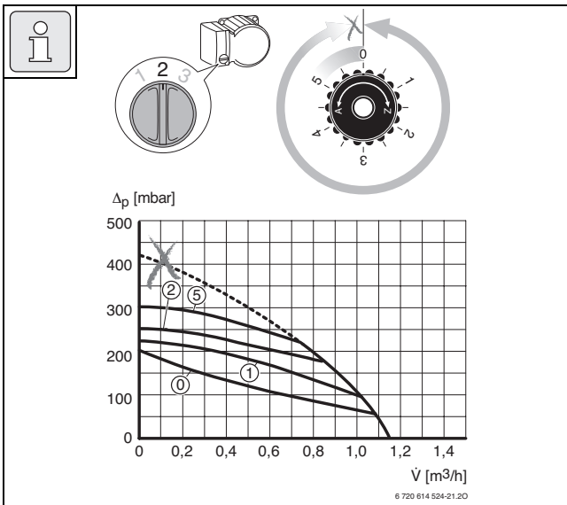
2.2 ZB 3/5-16 A, Z.B 7/11-22 A, ZWB 7/11-26 A
