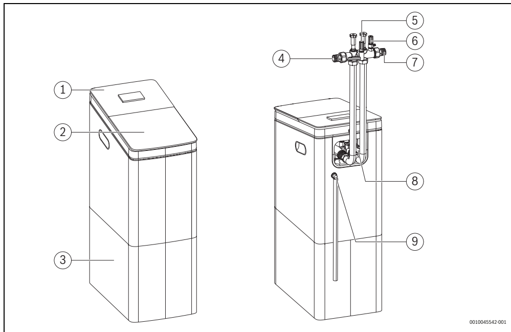
Fig. 5 Product overview
