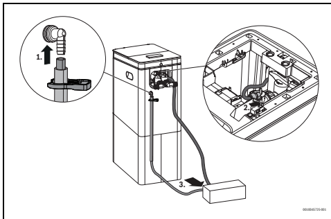
Fig. 11 Inserting hose on the overflow elbow
