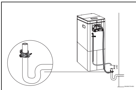
Fig. 12 Install the overflow pipe and drainpipe at the same time
