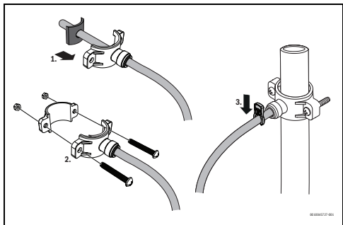
Fig. 14 Installation of the waste pipe clamp
