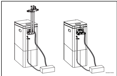
Fig. 13 Overview of the overflow elbow pipe and waste pipe after installation
