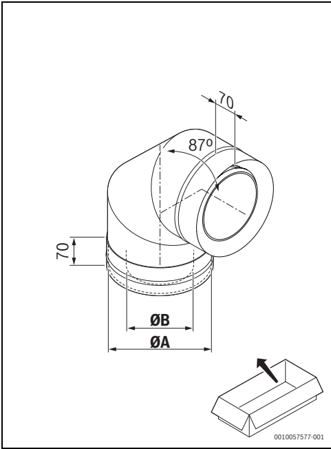
1 FC-CE125-87 / FC-CE160-87
