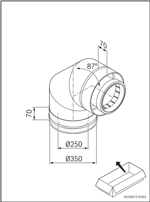
3 FC-CE250-87: 7738114043
