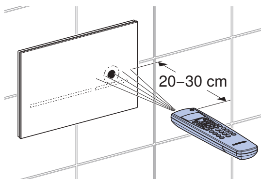
Ilustrimi 2: Operimi me Geberit Service-Handy
