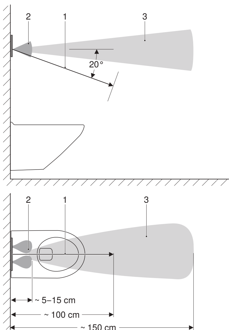
Figure 1: Detection ranges
