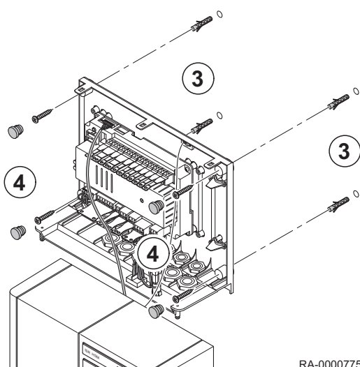
Abb.13 Wandmontage
