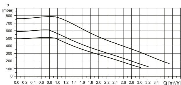
Abb. 27: UPM3 FLEX AS (Pufferladepumpe)
