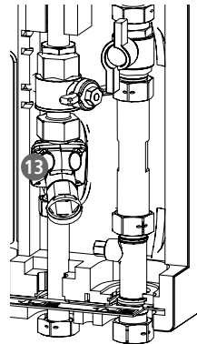
Abb. 10: AB-PM-Ventil
