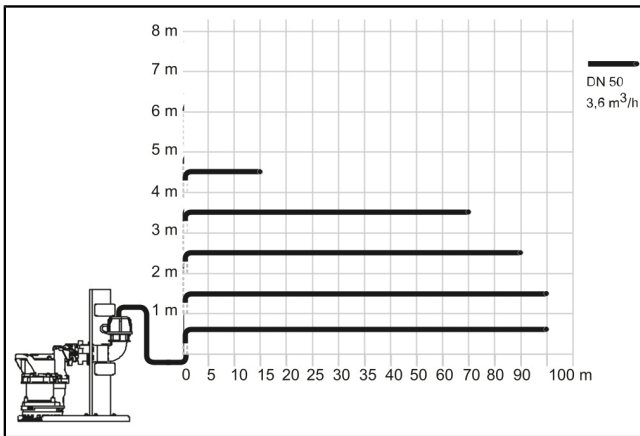
Fig.: Pumping performance diagram for Retrofit 500
