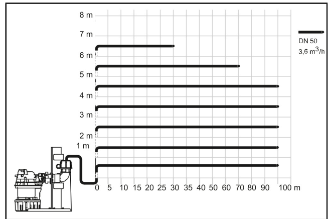
Fig.: Pumping performance diagram for Retrofit 1000
