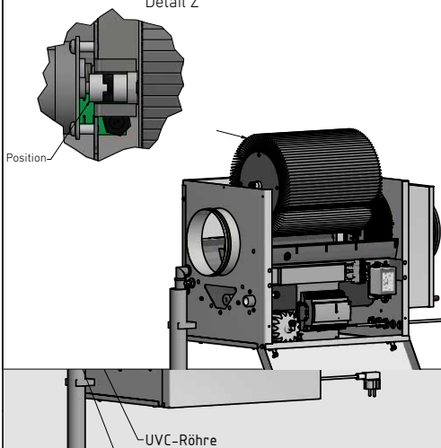
Detail Z
