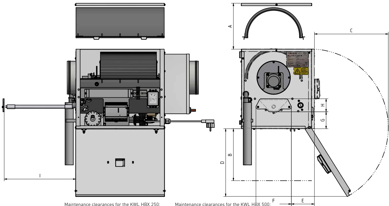
Maintenance clearances for the KWL HBX 250:
