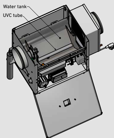
Detail Z
