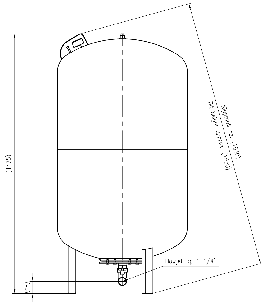
Side view
