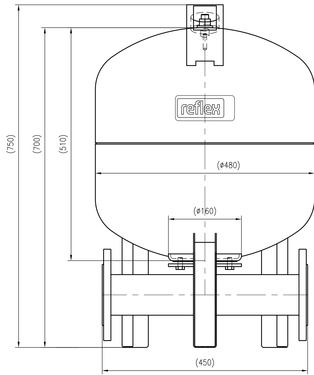
Front view
