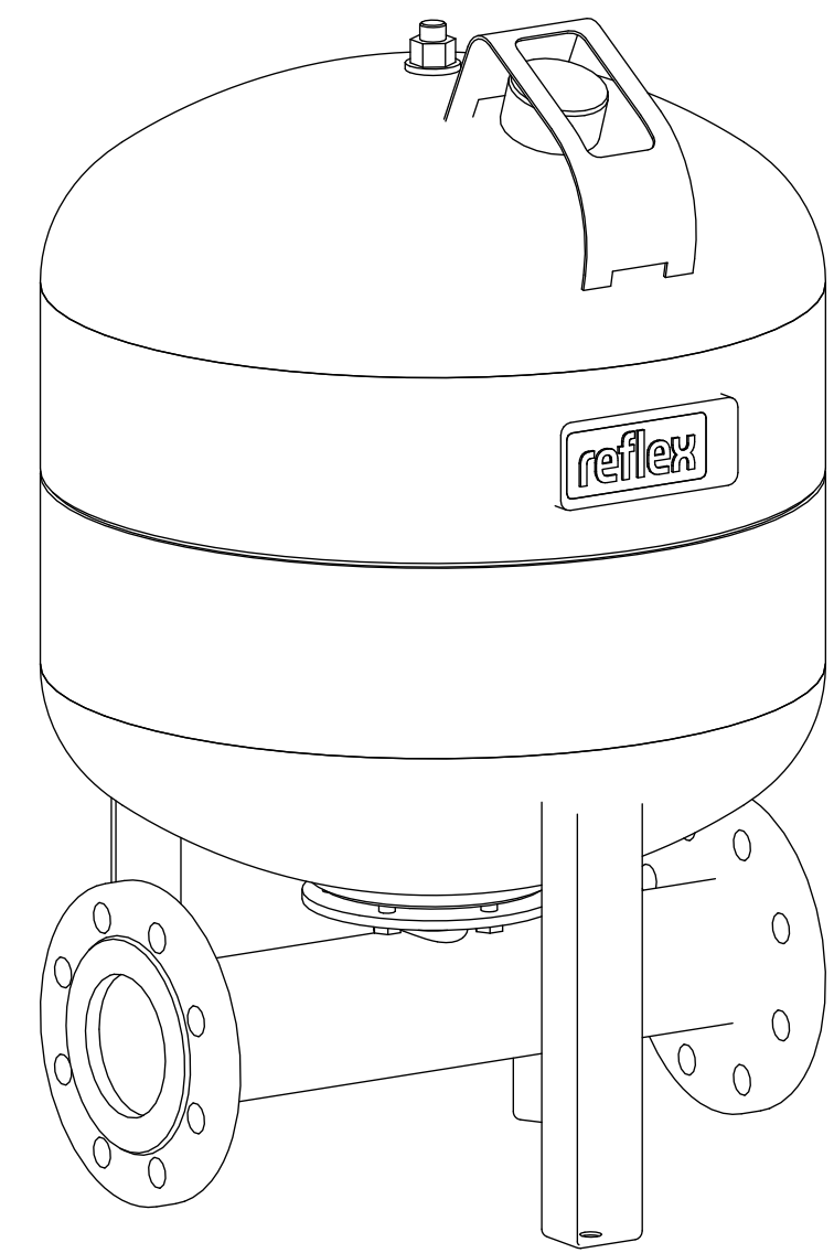
Isometric view
