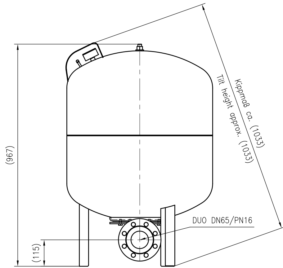
Side view
