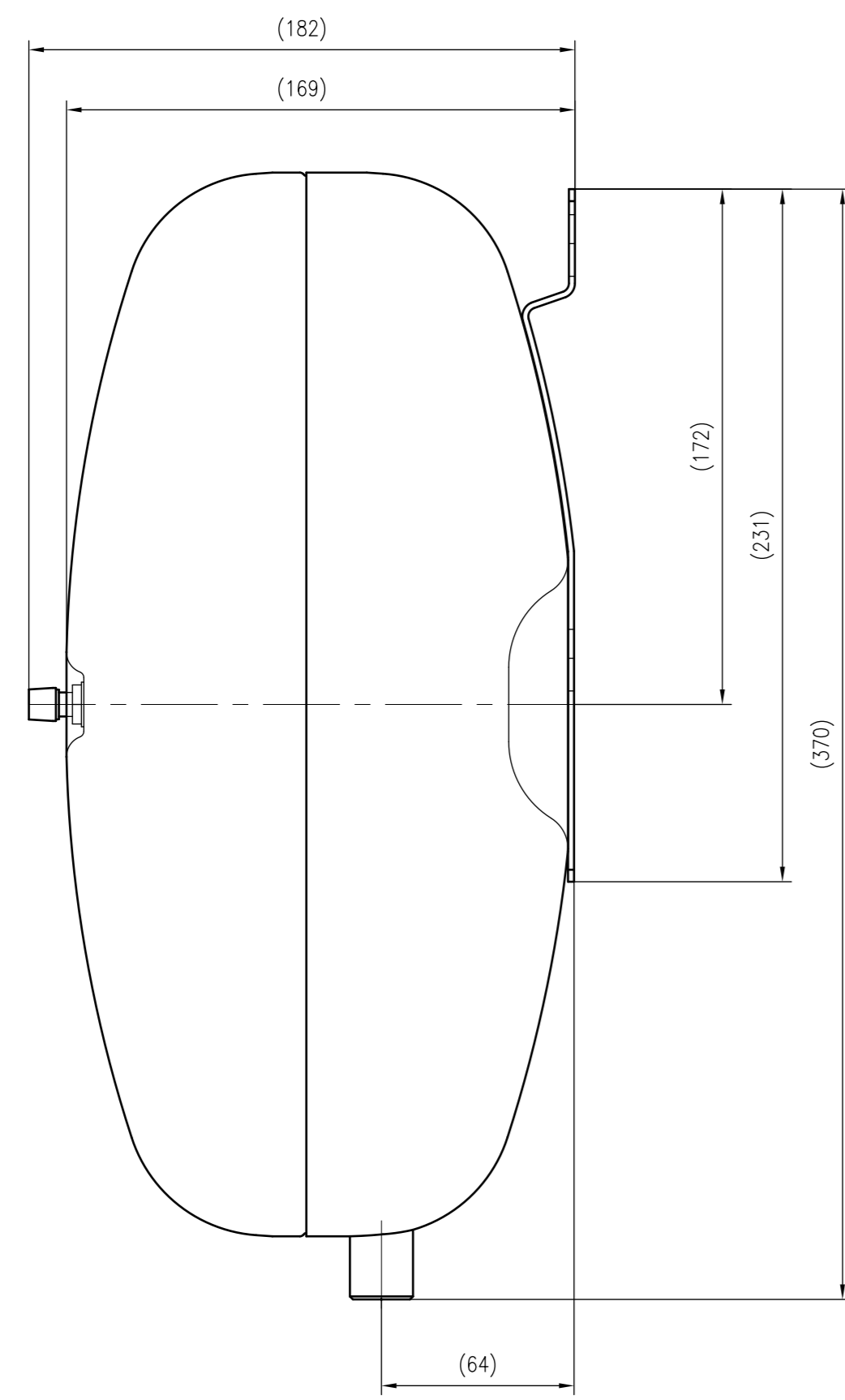
Side view
