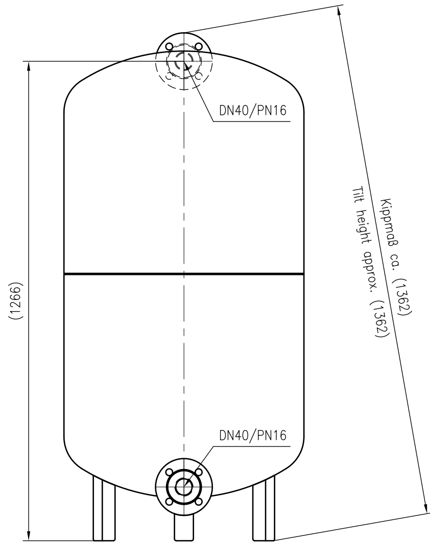
Side view
