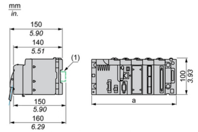
(1)AM1 ED rail (35x15), compatible only with BMXXBP0400/0400H/0600/0600H/0800/0800H racks
