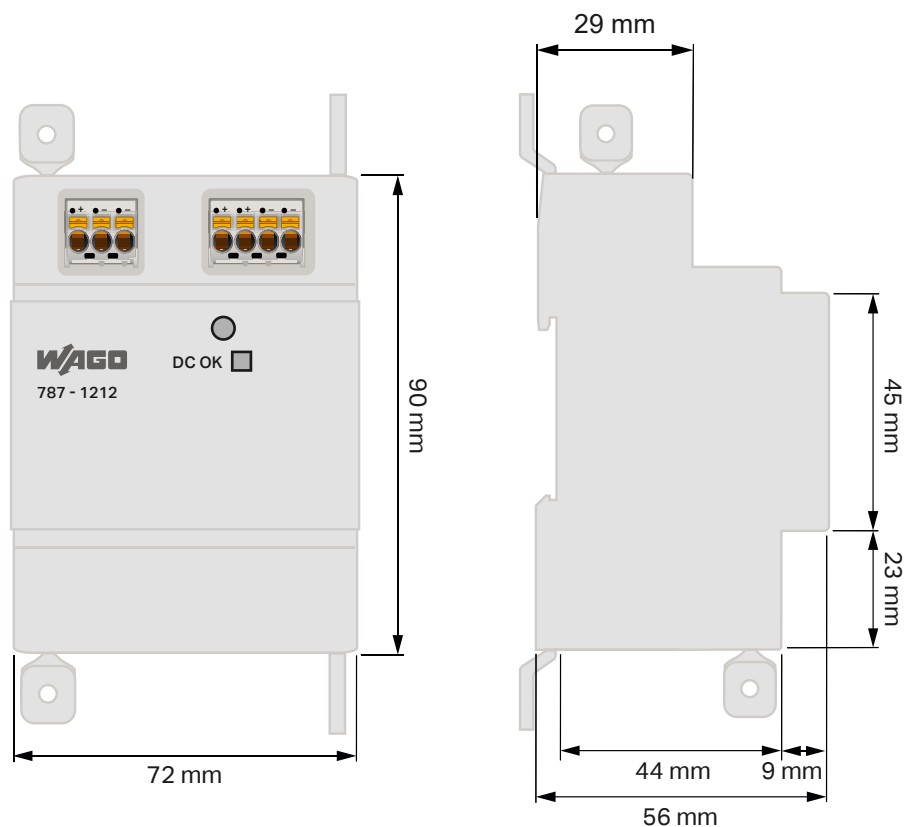
Fig. 7: Dimensions
