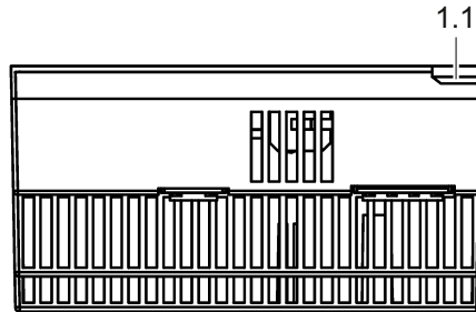
Figure 17: Snap-fit Openings for Fastening Clips – Top
