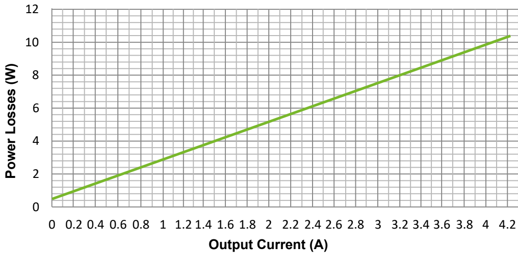
Figure 12: Power loss at 230 VAC
