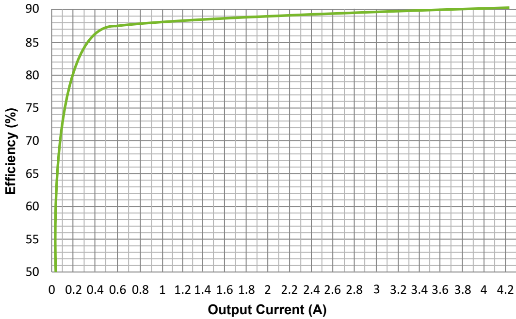
Figure 11: Efficiency at 230 VAC
