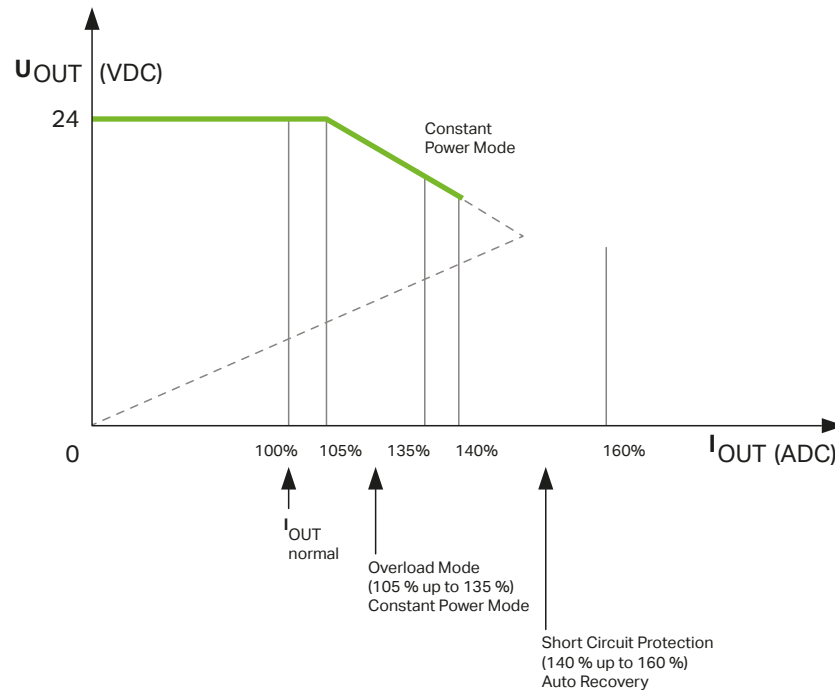
Figure 8: Overload Behavior
