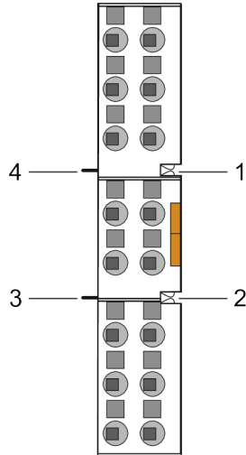
Figure 4: Power Jumper Contacts
