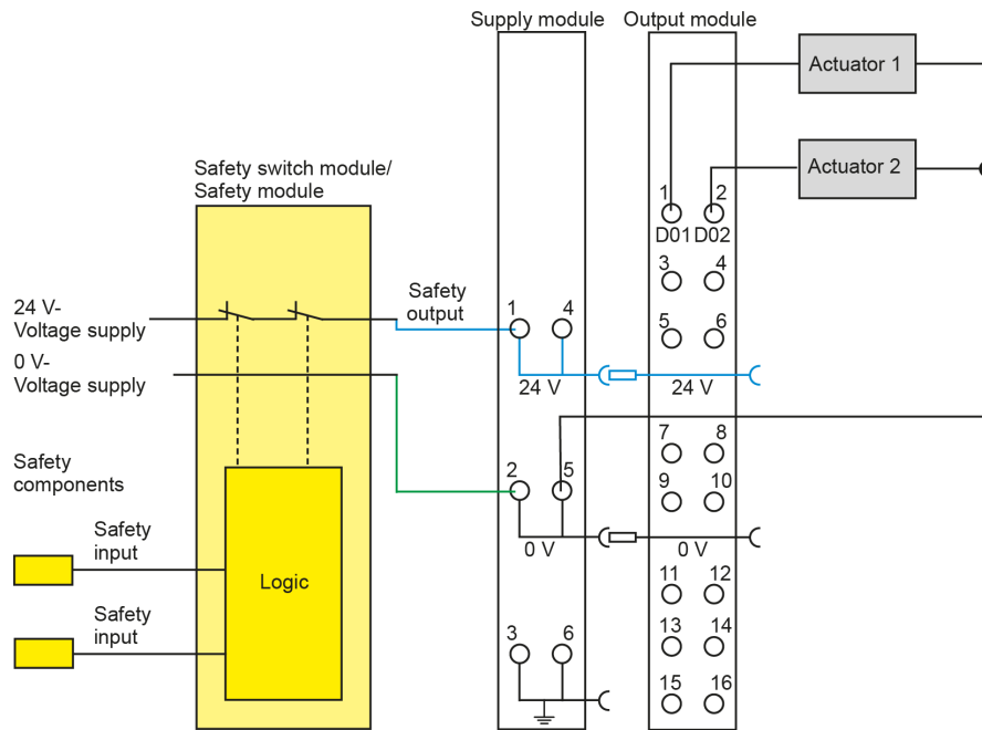
Figure 8: Two-Channel, Single-Pole Power Supply Shutdown
