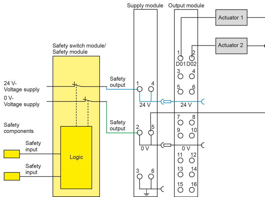
Figure 9: Two-Channel, Two-Pole Power Supply Shutdown
