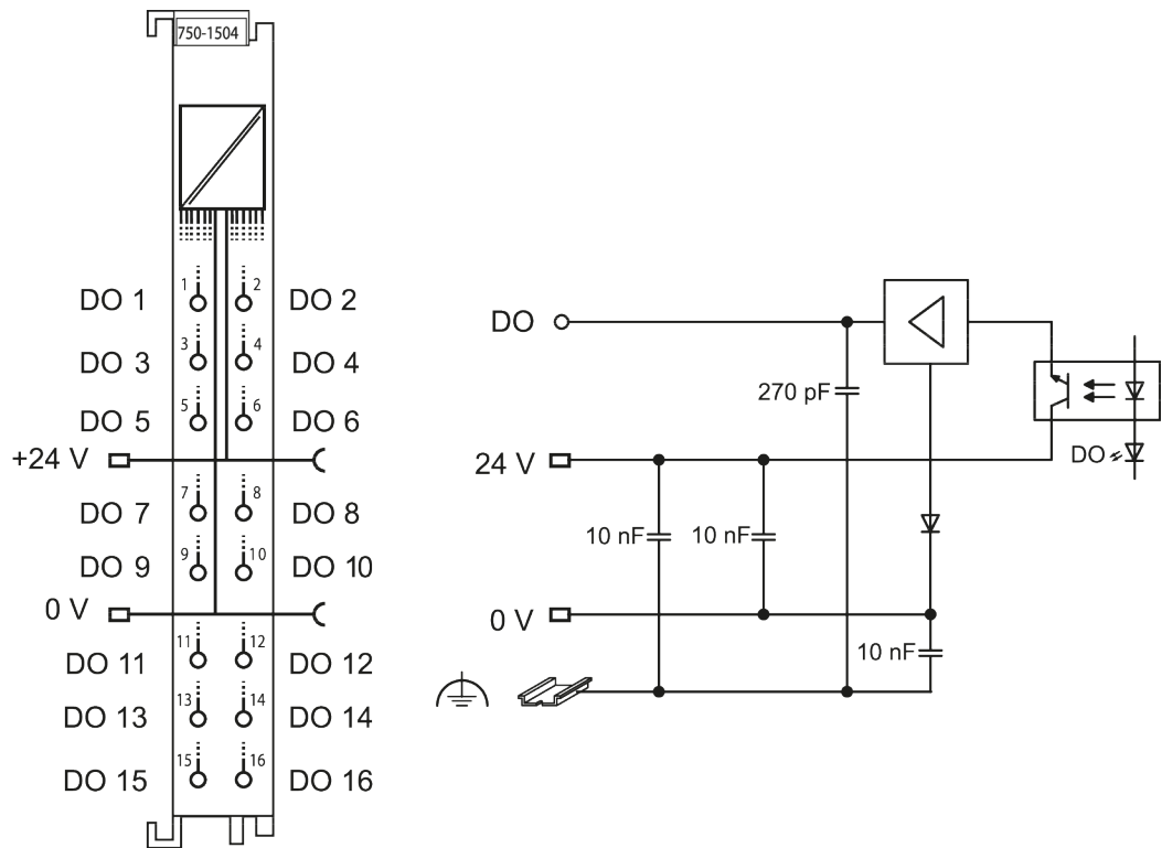
Figure 5: Circuit Diagram
