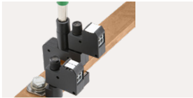
Installation on busbar; fastening with Allen wrench
