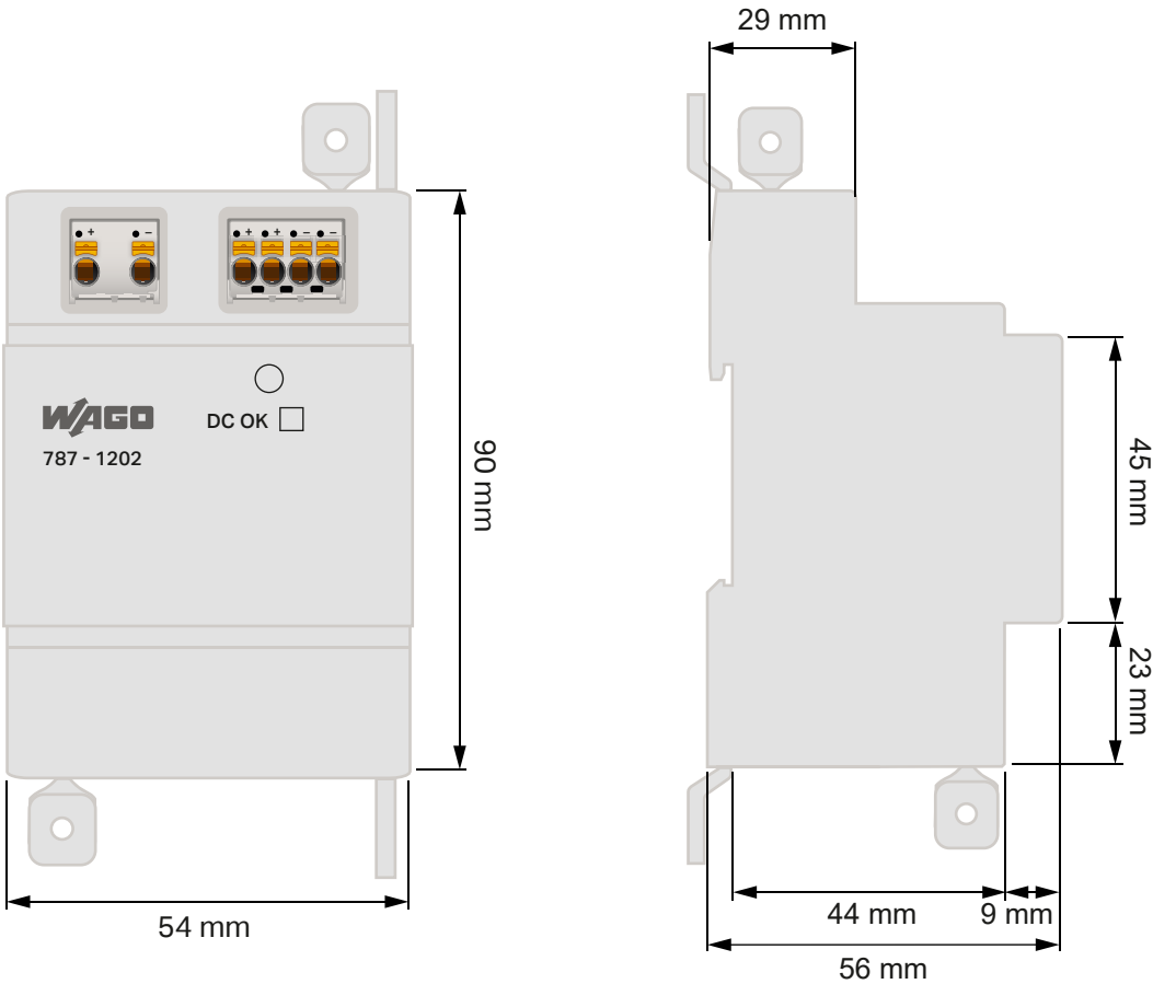
Fig. 7: Dimensions
