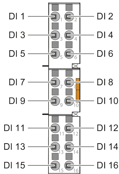
Figure 3: Push-in CAGE CLAMP ® connections
