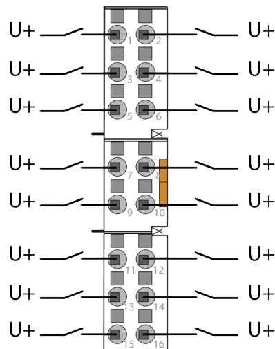
Figure 6: Example: 1-Wire Connection
