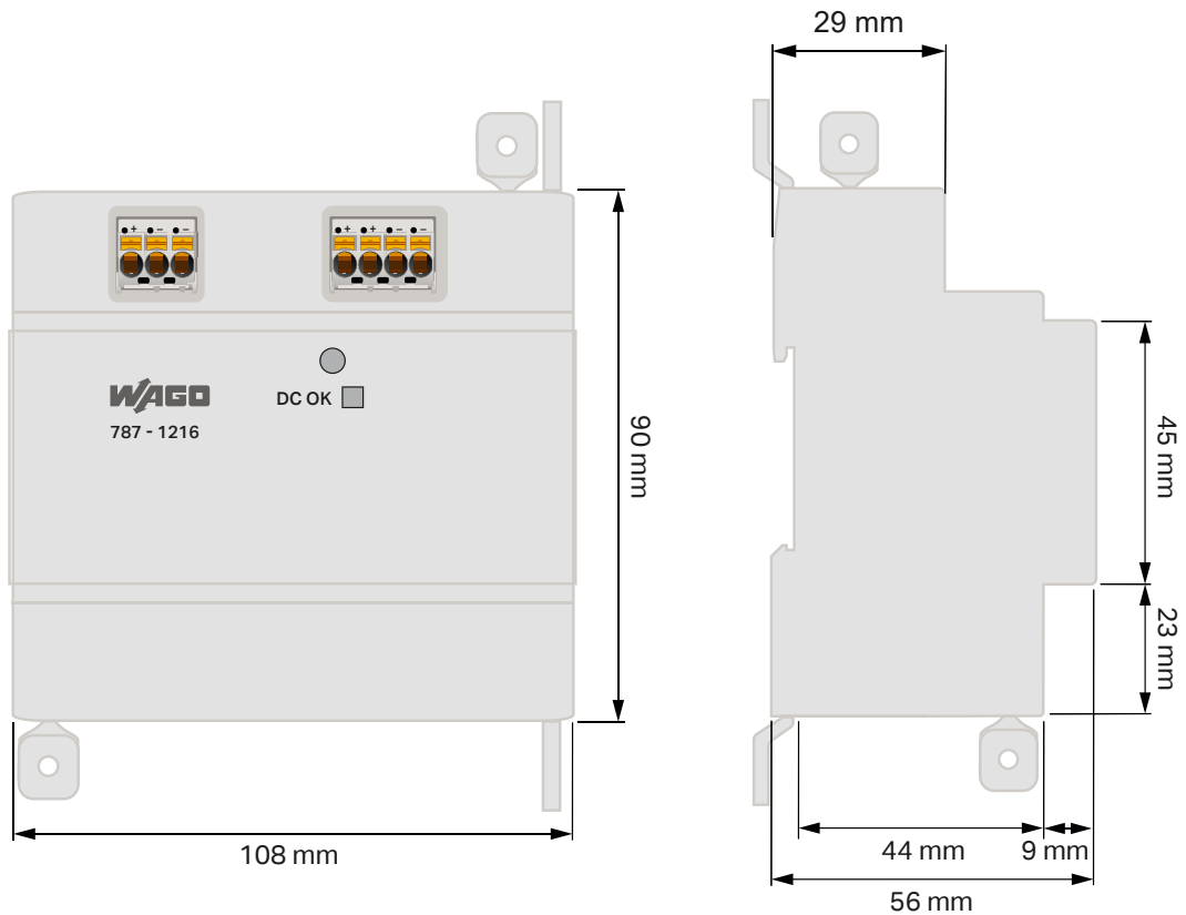
Fig. 7: Dimensions
