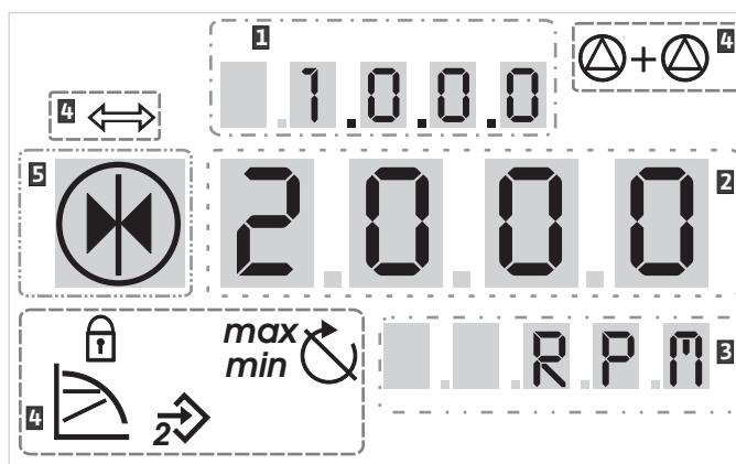
Fig. 29: Display structure
