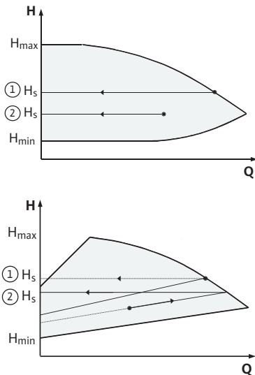
Fig. 42: Δp-c/Δp-v control
