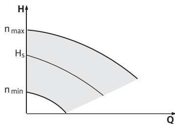
Fig. 43: Constant speed
