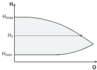
Fig. 10: Regulation \Delta p-c
