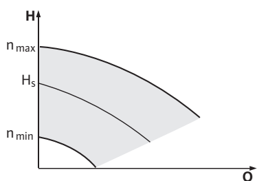
Fig. 12: Constant speed
