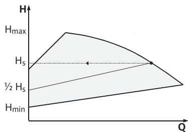
Fig. 11: Regulation \Delta p-v
